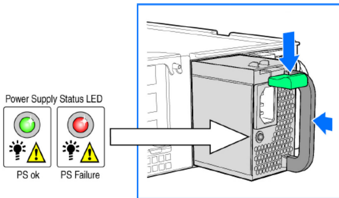
FIGURE 392 Replacing a PSU
