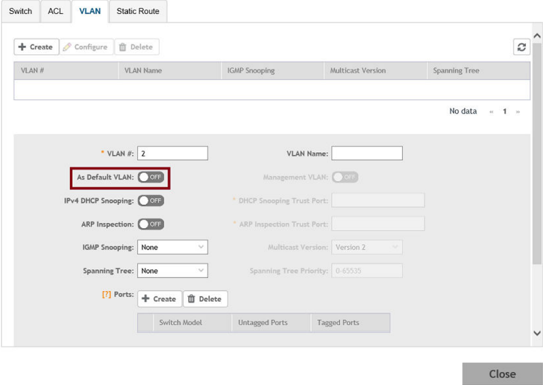
FIGURE 119 VLAN Configuration
