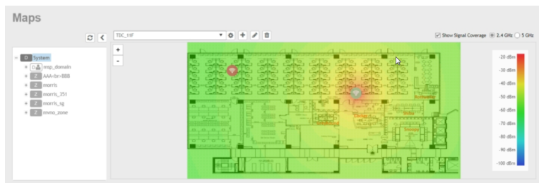
FIGURE 91 RF Coverage Heat Map
